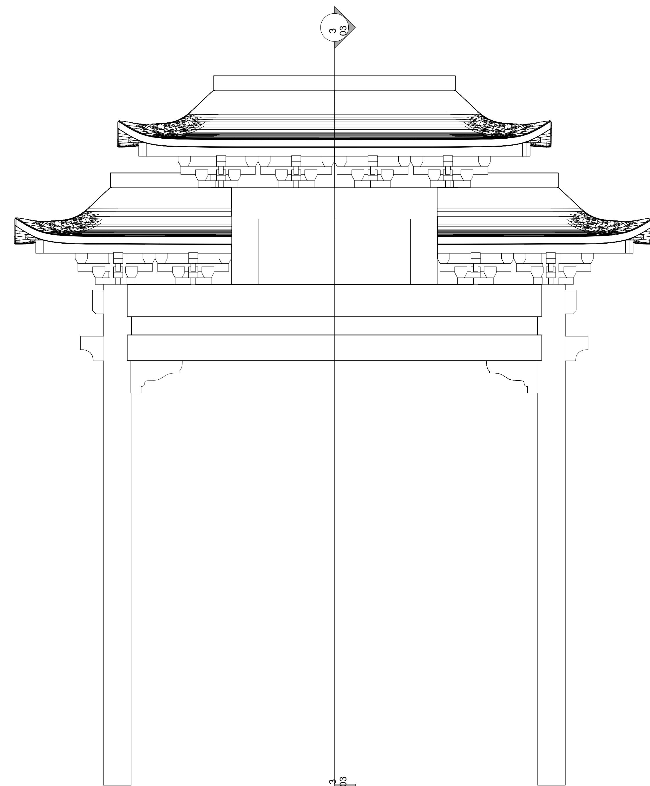
2 Temple roof facade elevation Scale: 1/2" = 1'-0"
