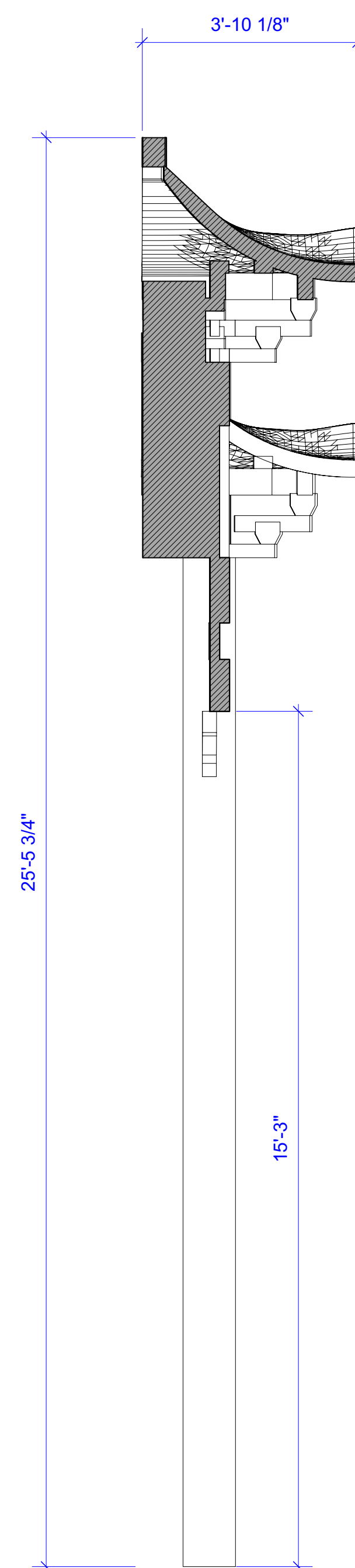
3 Temple roof facade section Scale: 1/2" = 1'-0"
