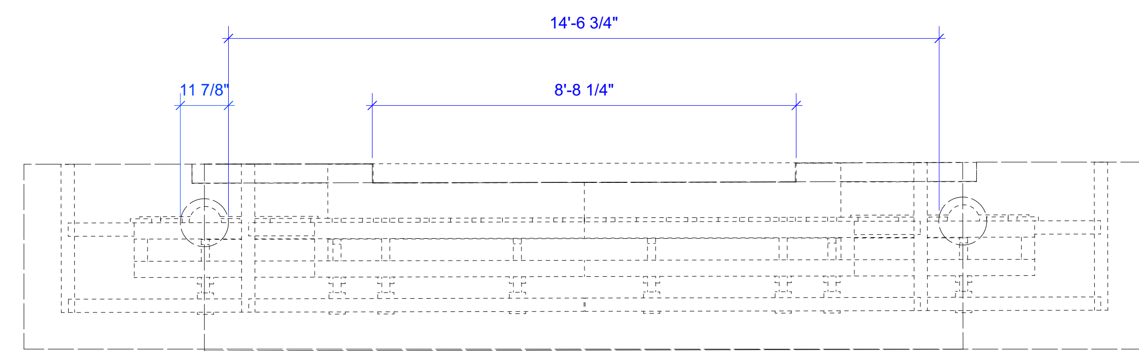
1 Temple roof facade plan Scale: 1/2" = 1'-0"
