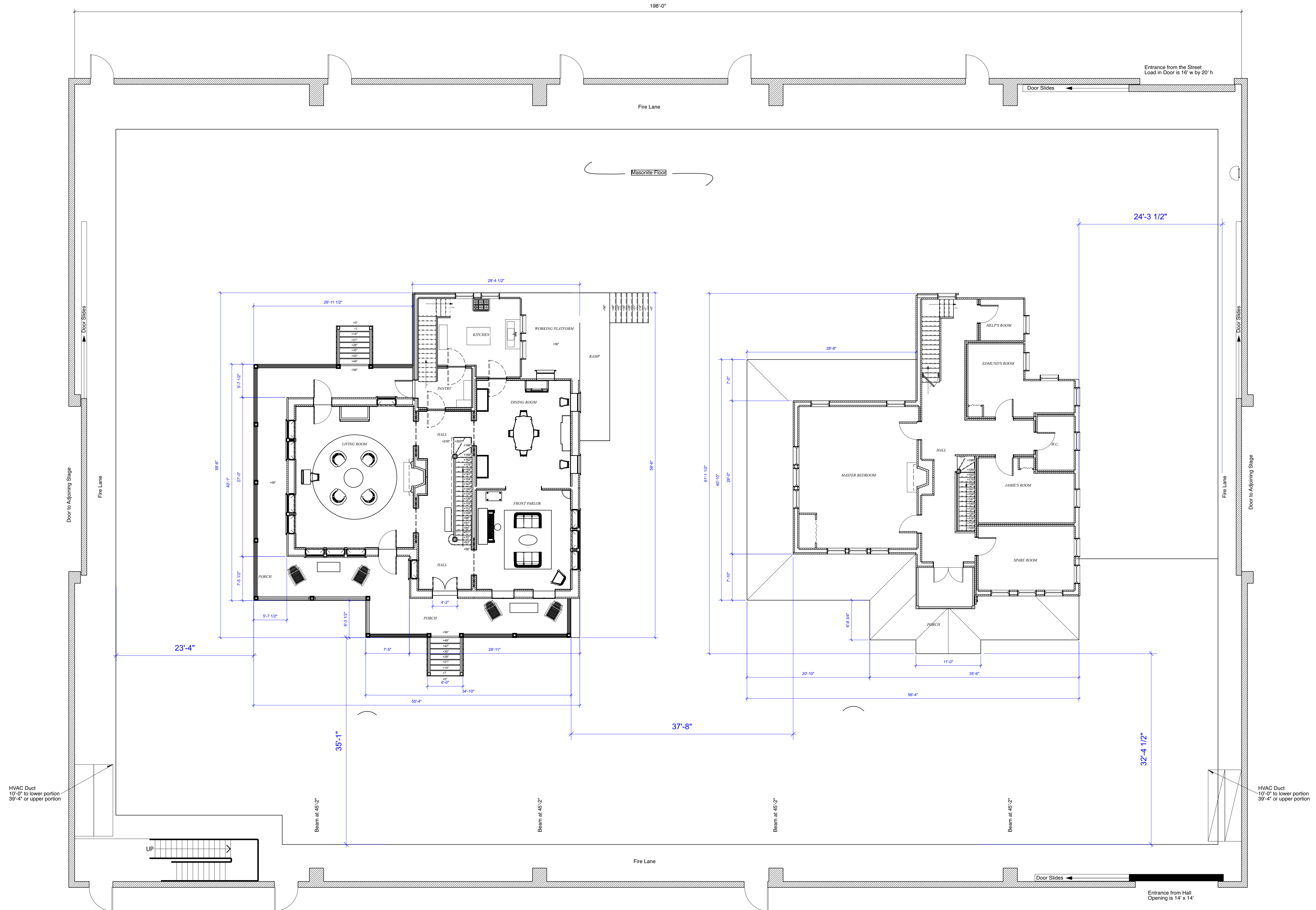
Steiner Studios Stage 3 Plan Scale: 1/8" = 1'-0"
